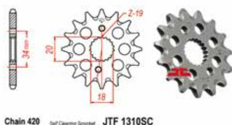
Chain 420 Self-Cleaning Sprocket JTF 1310SC
